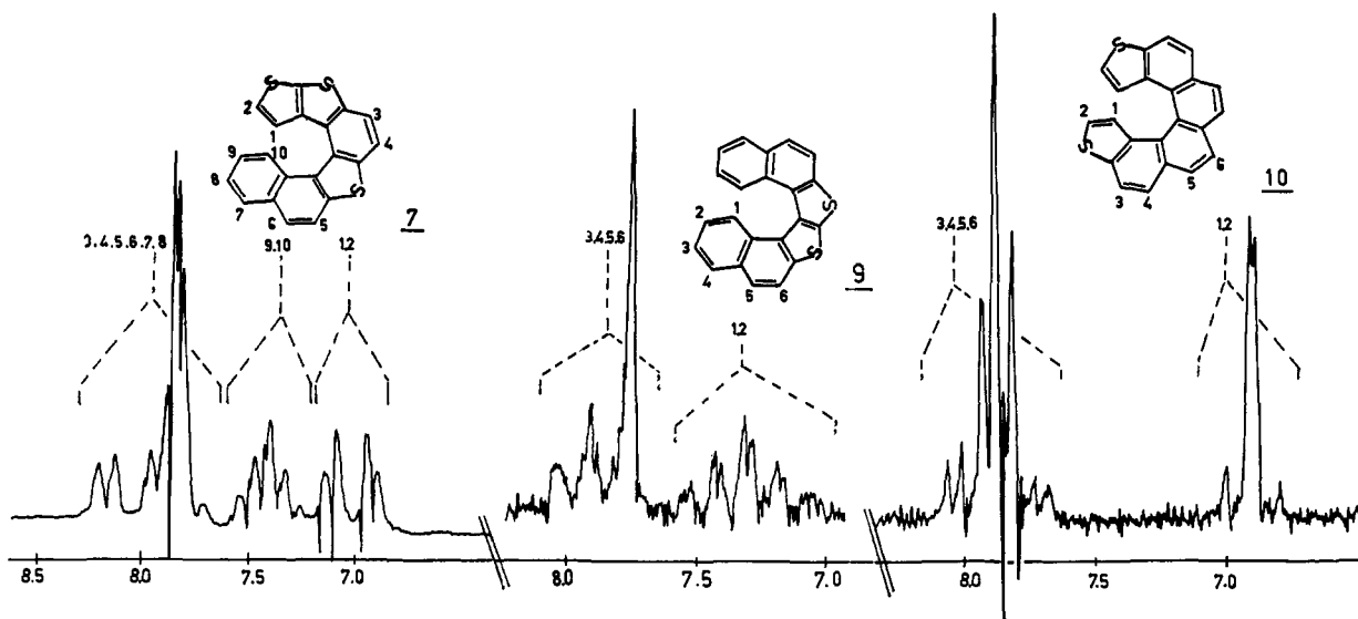
Figure 2. Nmr spectra of 7, 9, and 10 in \text{CS}_2 .
