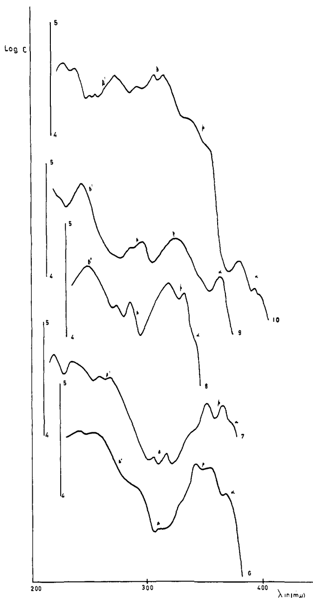
Figure 3. Uv spectra of the helicenes 6-10 in \text{C}_6\text{H}_{12} .
