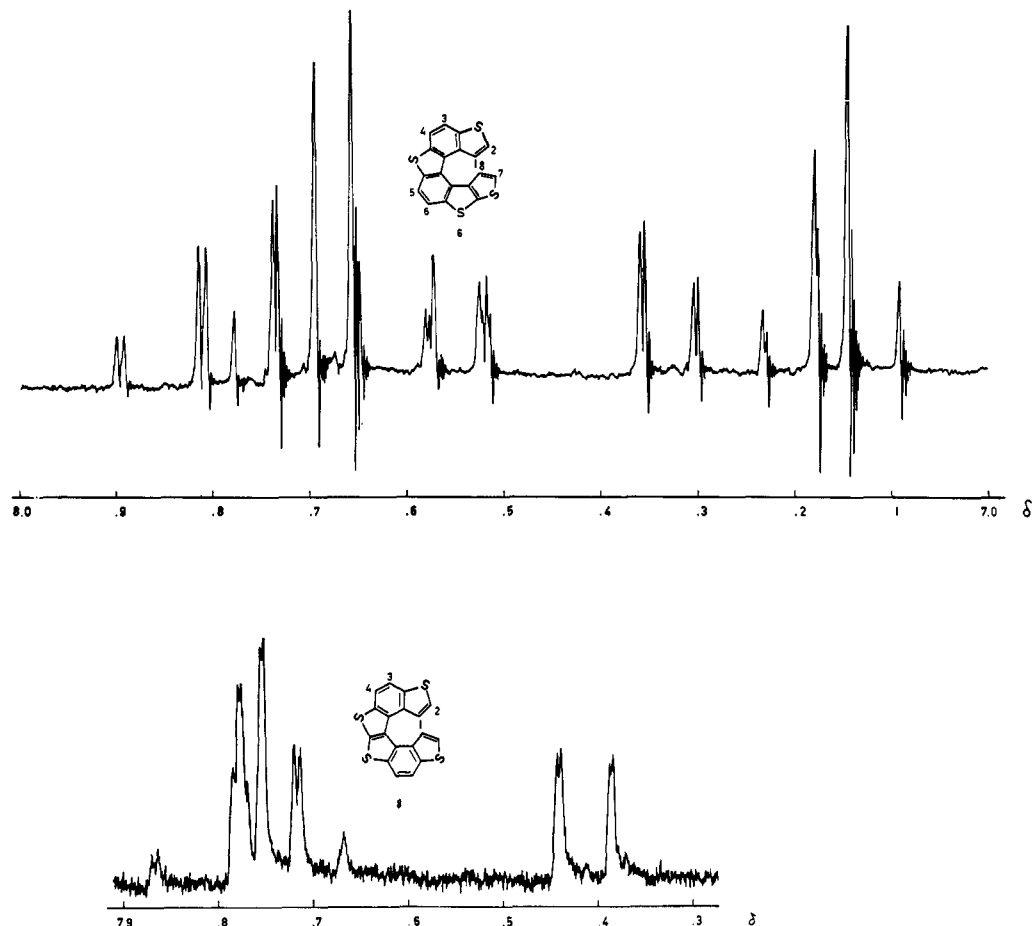
Figure 1. 100-MHz nmr spectra of 6 and 8 in \text{CS}_2 .
